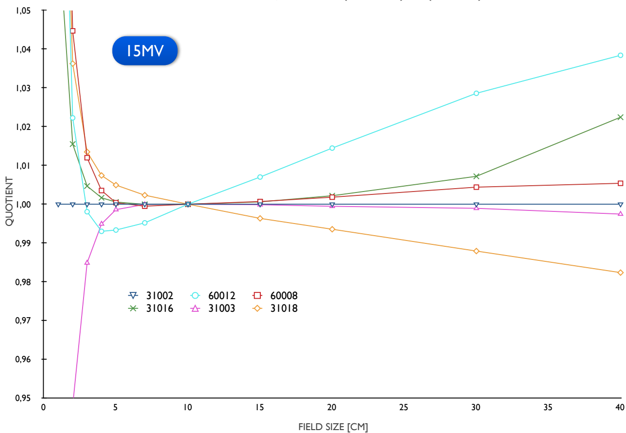
OUTPUT FACTOR QUOTIENT: OF(DETECTOR) / OF(31002-368)
